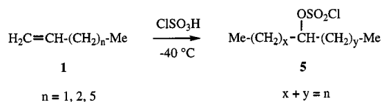
Scheme 3. Reaction of the \alpha -olefins 1b , 1g , and 1h with ClSO 3 H in CDCl 3 at -40^\circ\text{C}
