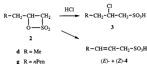
Scheme 2. Conversion of the 1,2-alkanesultones 2 in the presence of HCl into the corresponding 1-alkane-2-chlorosulfonic acids 3 , and the ( E )- and ( Z )-2-alkene-1-sulfonic acids 4
