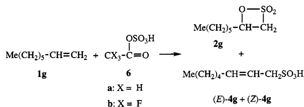
Scheme 5. Reaction of 1-octene ( 1g ) with acetyl sulfate ( 6a ) and trifluoroacetyl sulfate ( 6b ) in \text{CDCl}_3
