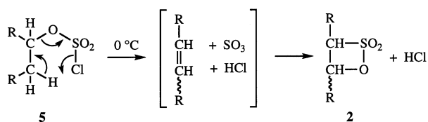
Scheme 4. Mechanism for the conversion of sec -alkyl chlorosulfates 5 into the \beta -sultones 2 in \text{CDCl}_3
